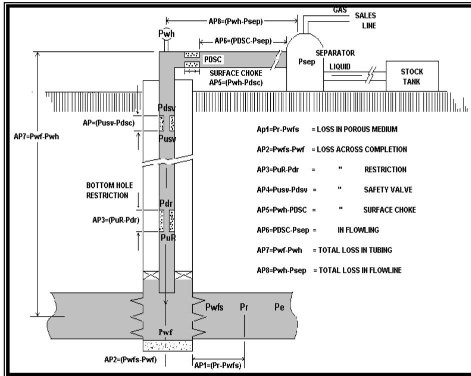
Figure 4. Oil Well Production System
