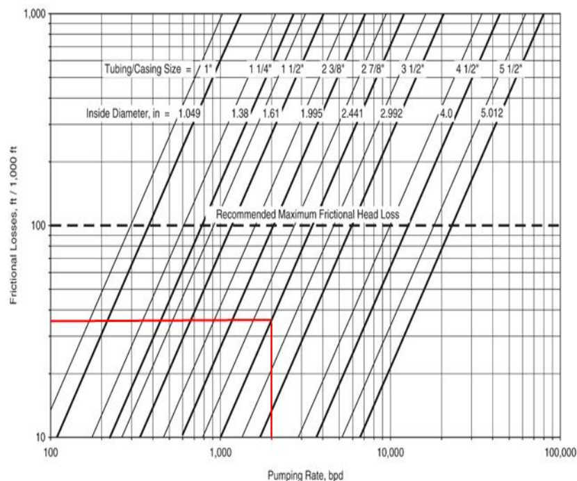
Figure 5. Friction Loss Hazen-William Graph
